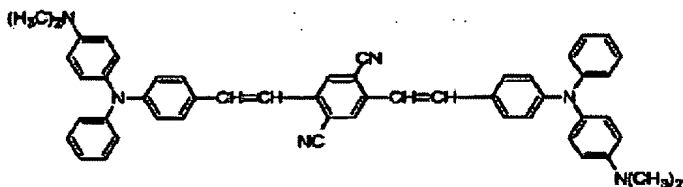
Structural formula (15)-5:
